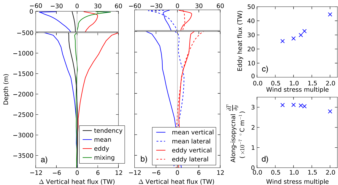
Figure 3. Heat flux response in the southern region ( 40\text{--}70^\circ\text{S} only) to a 30% increase in Southern Ocean wind stress. (a) Change from the equilibrium vertical heat fluxes (net heat divergence) in the southern region, averaged over the first 10 years of the perturbation. Heat flux components (colors) are defined as in Figure 1, with the additional heat content tendency, \mathcal{T} (black). (b) Separation of the net mean and eddy heat fluxes shown in Figure 3a into true vertical (solid lines) and lateral (dashed lines) components. (c) Scaling of the net eddy heat flux in the southern region, averaged over the depth range 700–1600 m. (d) Scaling of the along-isopycnal, meridional temperature gradient on a mid-depth isopycnal (1500 m depth at 42^\circ\text{S} , 700 m depth at 62^\circ\text{S} ).
