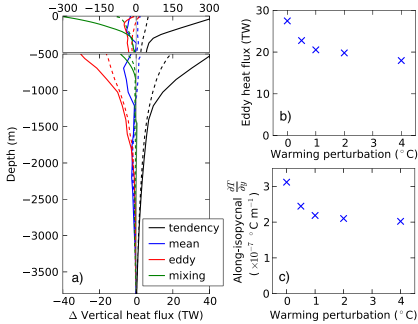
Figure 2. Vertical heat flux response to a uniform +2^\circ\text{C} warming perturbation. (a) Change from the equilibrium vertical heat fluxes, averaged over the first 10 years of the perturbation, integrated over the entire domain (solid lines) and the contribution from the southern region (dashed lines). Heat flux components (colors) are defined as in Figure 1, with the additional heat content tendency, \mathcal{T} (black). (b) Scaling of the vertical eddy heat flux in the southern region (i.e., the blue line in Figure 1b), averaged over the depth range 700–1600 m. (c) Scaling of the along-isopycnal, meridional temperature gradient on a mid-depth isopycnal (1500 m depth at 42^\circ\text{S} , 700 m depth at 62^\circ\text{S} ).
